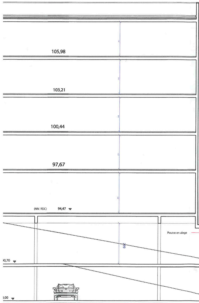
COUPE FACADE AA
